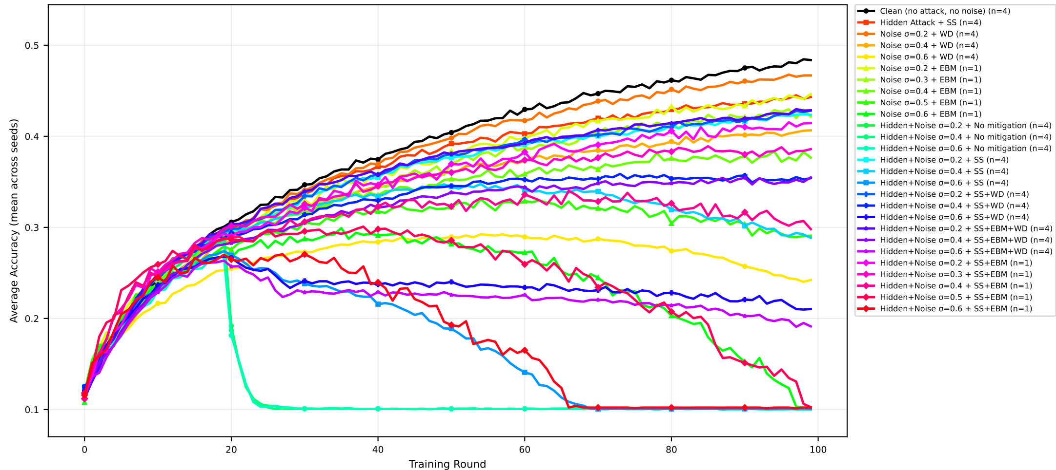
Zoomed Accuracy | CIFAR-10 | MERGED | Overall Average (nonIID)
